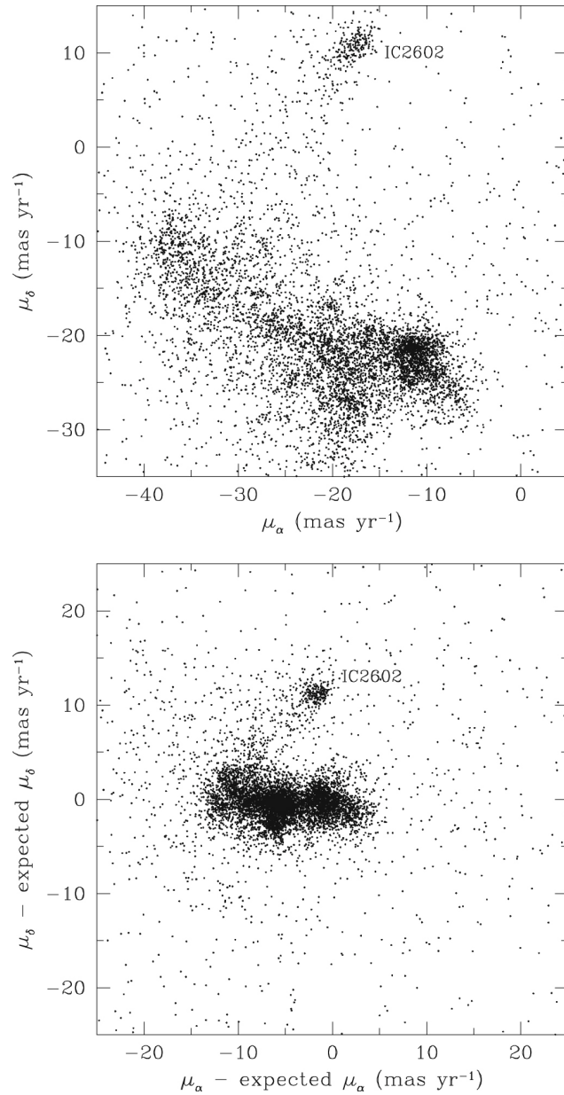
Figure 3. from Refining the Census of the Upper Scorpius Association with Gaia null 2020 AJ 160 44 doi:10.3847/1538-3881/ab9599 https://dx.doi.org/10.3847/1538-3881/ab9599 © 2020. The American Astronomical Society. All rights reserved.
