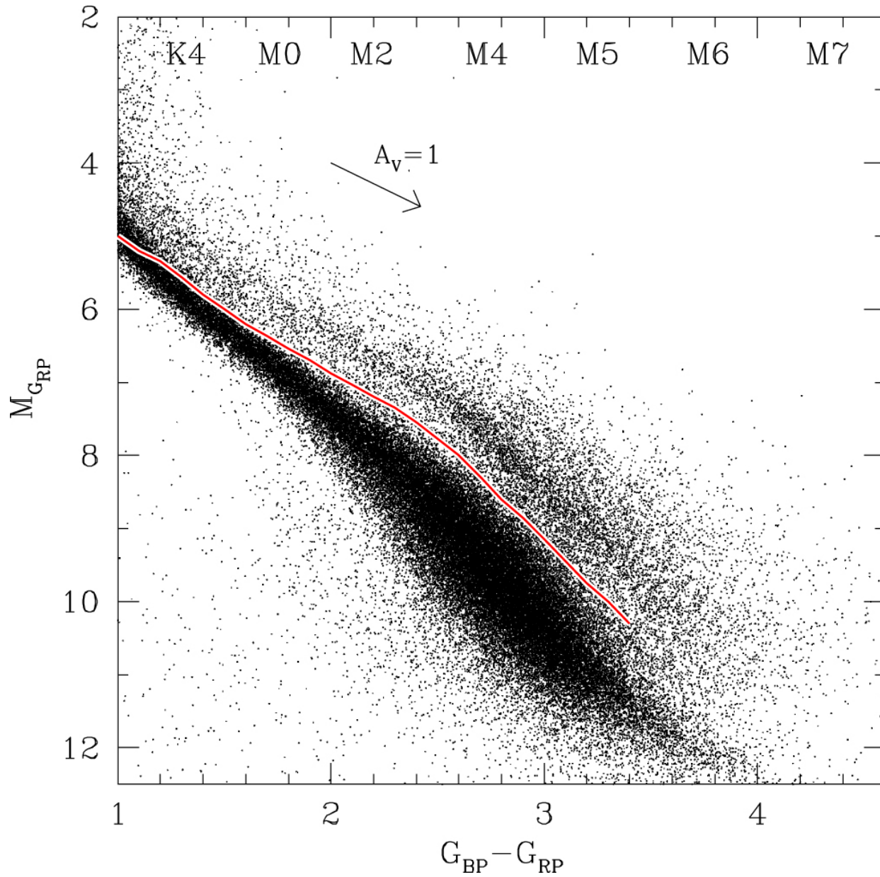
Figure 2. from Refining the Census of the Upper Scorpius Association with Gaia null 2020 AJ 160 44 doi:10.3847/1538-3881/ab9599 http://dx.doi.org/10.3847/1538-3881/ab9599 © 2020. The American Astronomical Society. All rights reserved.
