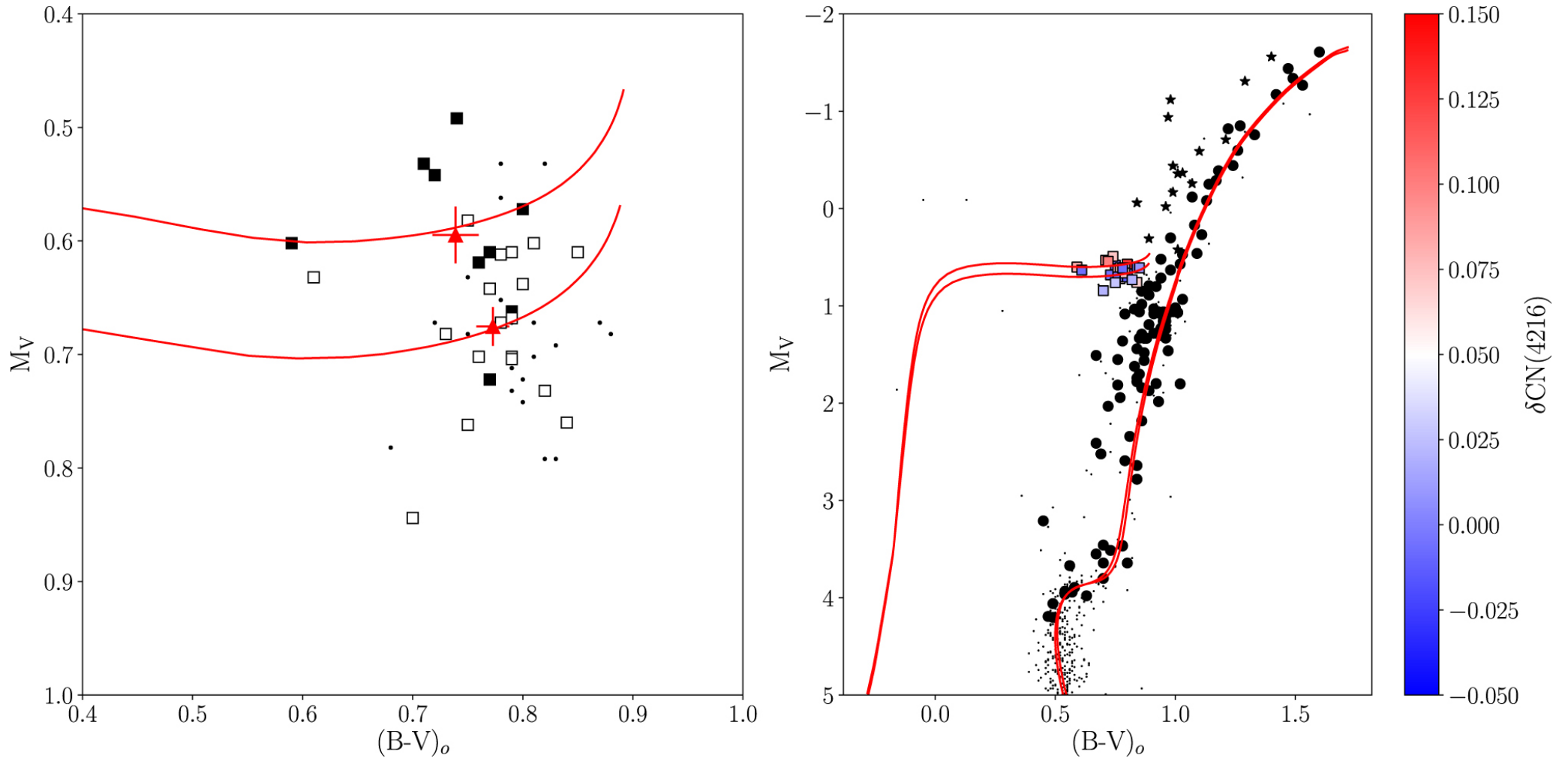
Figure 7. from Identifying Multiple Populations in M71 Using CN null 2020 AJ 159 50 doi:10.3847/1538-3881/ab607e https://dx.doi.org/10.3847/1538-3881/ab607e © 2020. The American Astronomical Society. All rights reserved.
