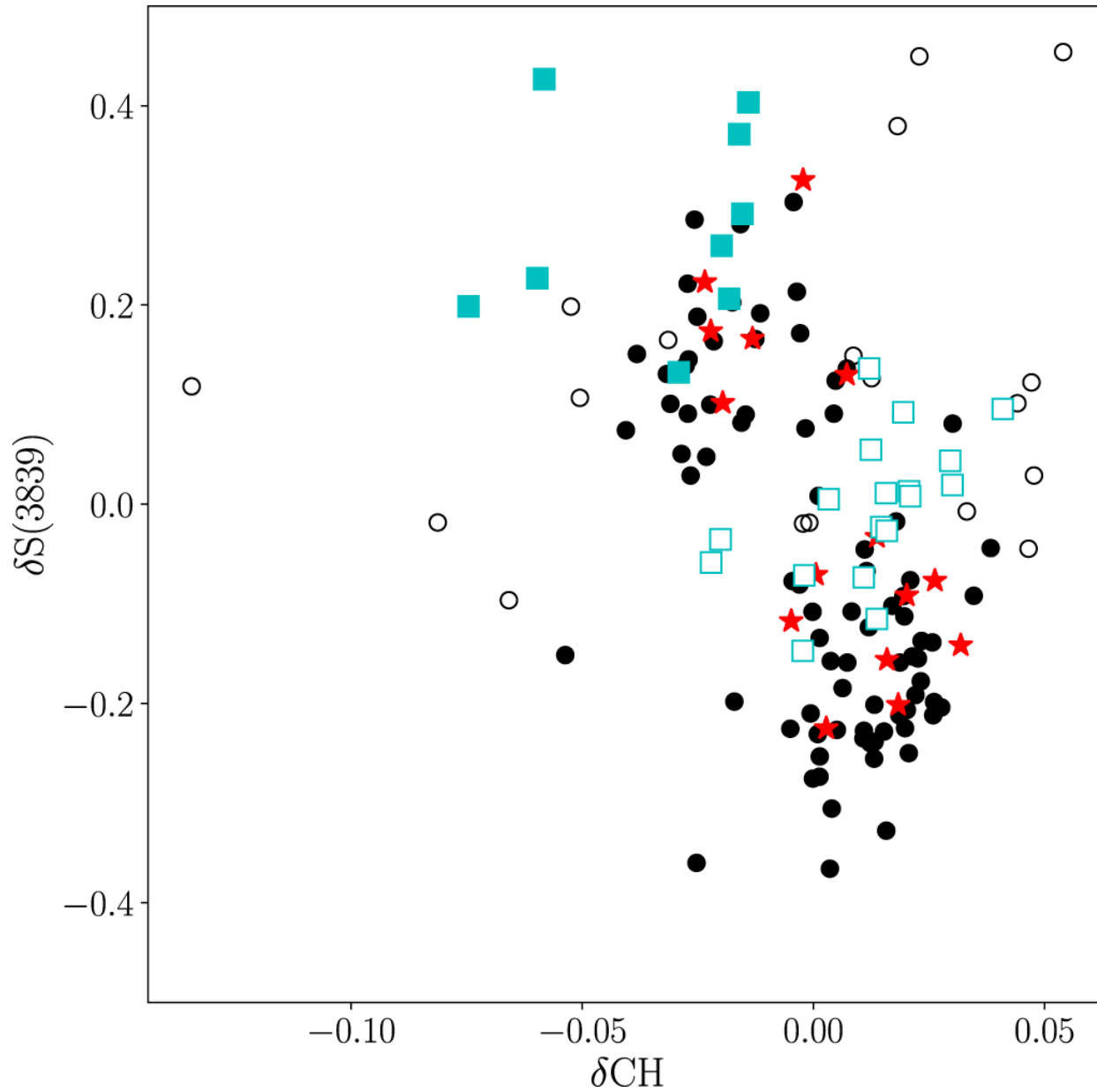
Figure 6. from Identifying Multiple Populations in M71 Using CN null 2020 AJ 159 50 doi:10.3847/1538-3881/ab607e http://dx.doi.org/10.3847/1538-3881/ab607e © 2020. The American Astronomical Society. All rights reserved.
