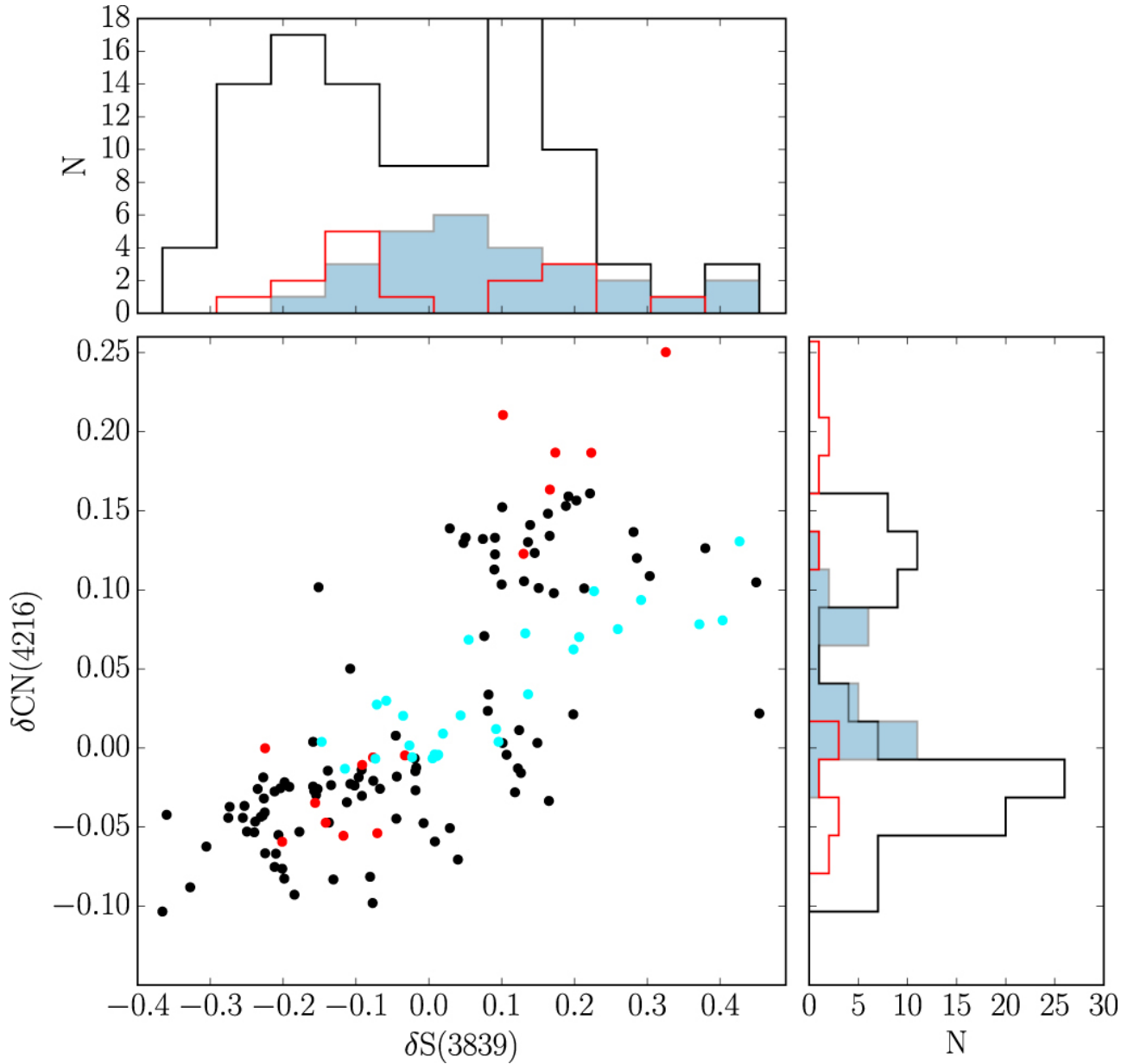
Figure 4. from Identifying Multiple Populations in M71 Using CN null 2020 AJ 159 50 doi:10.3847/1538-3881/ab607e http://dx.doi.org/10.3847/1538-3881/ab607e © 2020. The American Astronomical Society. All rights reserved.
