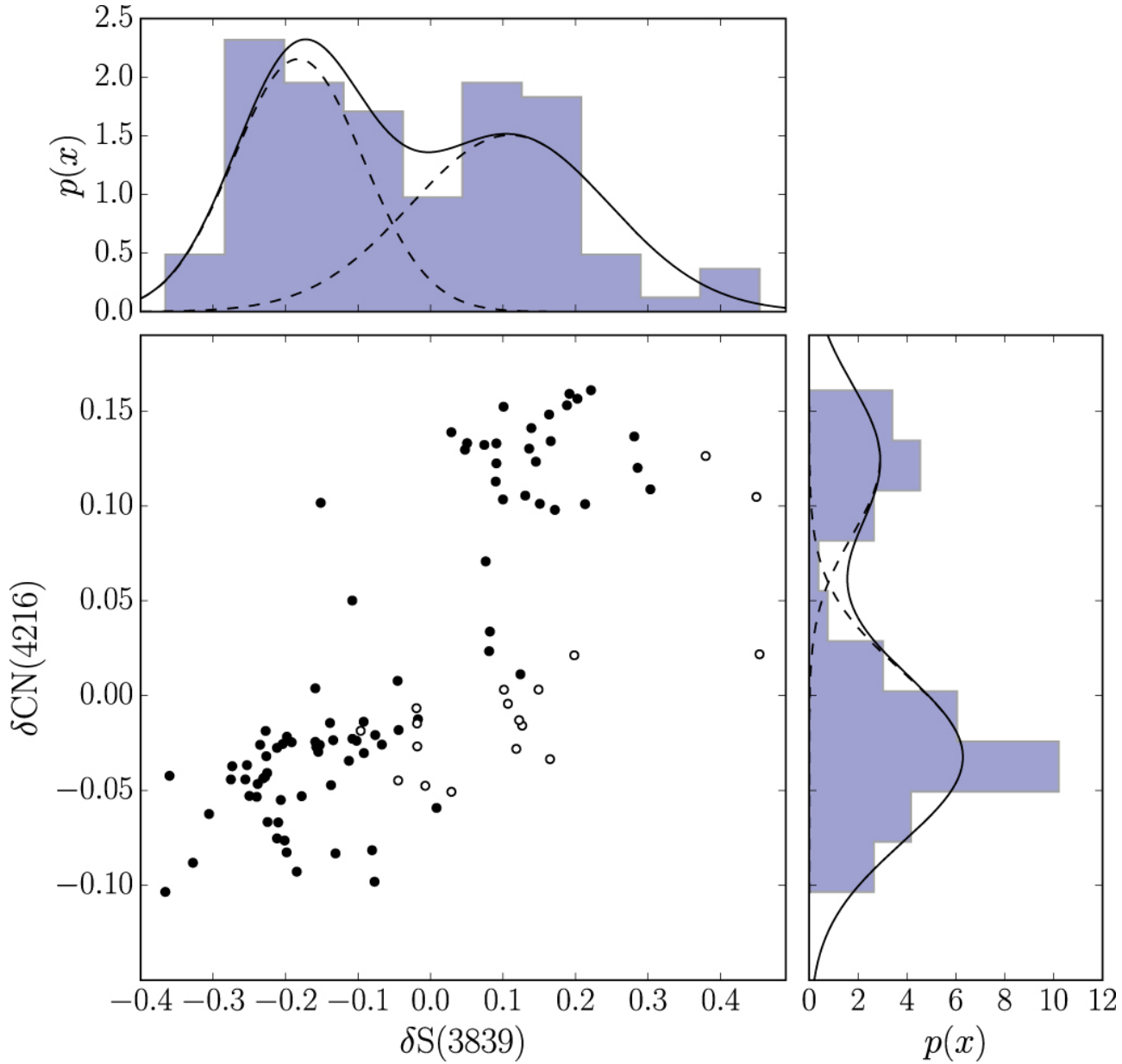
Figure 3. from Identifying Multiple Populations in M71 Using CN null 2020 AJ 159 50 doi:10.3847/1538-3881/ab607e http://dx.doi.org/10.3847/1538-3881/ab607e © 2020. The American Astronomical Society. All rights reserved.
