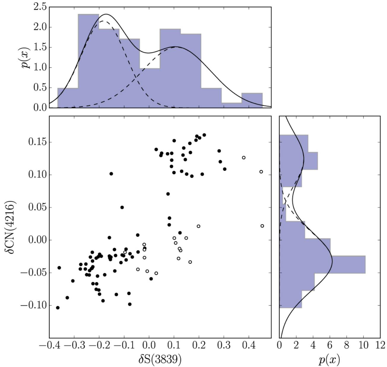
Figure 3. from Identifying Multiple Populations in M71 Using CN null 2020 AJ 159 50 doi:10.3847/1538-3881/ab607e https://dx.doi.org/10.3847/1538-3881/ab607e
