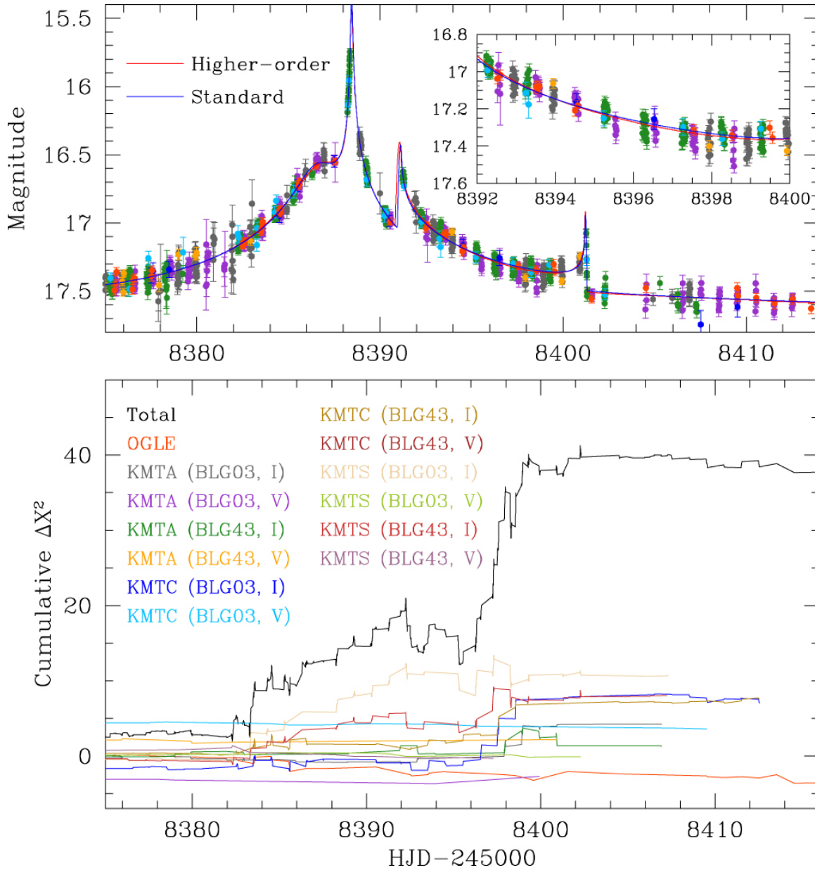
Figure 5. from OGLE-2018-BLG-1700L: Microlensing Planet in Binary Stellar System null 2020 AJ 159 48 doi:10.3847/1538-3881/ab5db9 http://dx.doi.org/10.3847/1538-3881/ab5db9 © 2020. The American Astronomical Society. All rights reserved.
