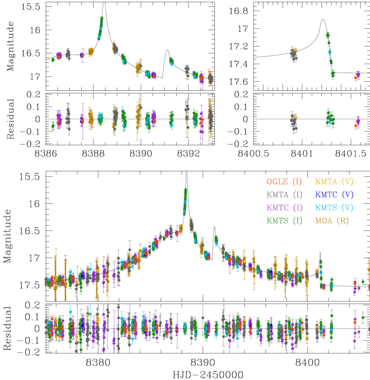
Figure 3. from OGLE-2018-BLG-1700L: Microlensing Planet in Binary Stellar System null 2020 AJ 159 48 doi:10.3847/1538-3881/ab5db9 http://dx.doi.org/10.3847/1538-3881/ab5db9
