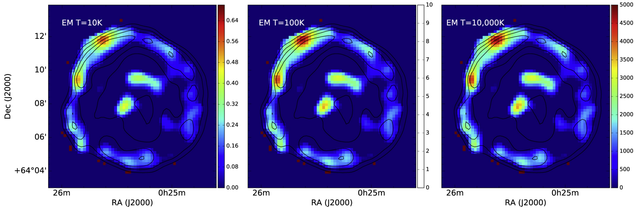
Figure 8. from Low-frequency Radio Absorption in Tycho's Supernova Remnant null 2019 AJ 158 253 doi:10.3847/1538-3881/ab4f80 https://dx.doi.org/10.3847/1538-3881/ab4f80 © 2019. The American Astronomical Society. All rights reserved.
