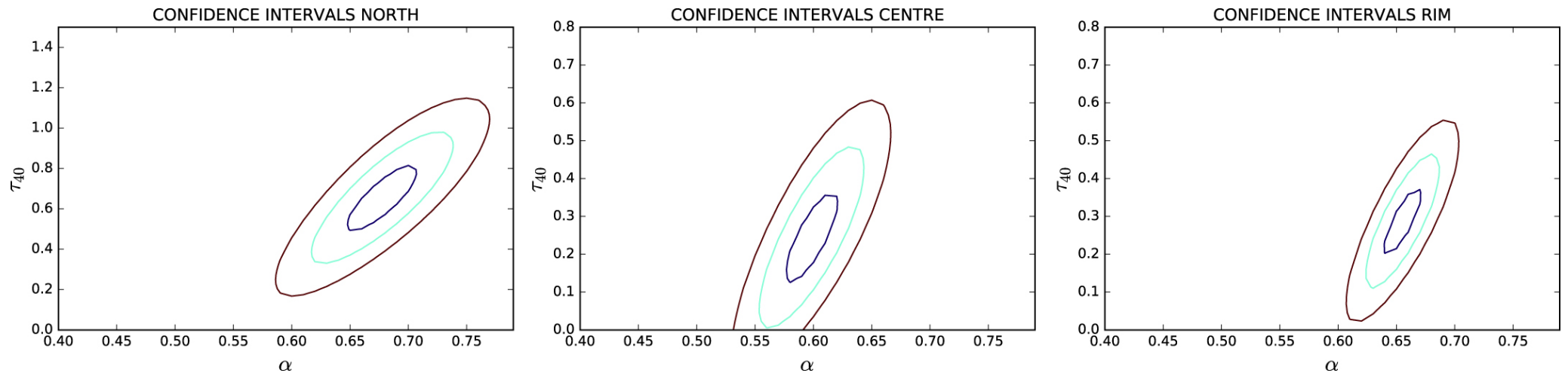
Figure 7. from Low-frequency Radio Absorption in Tycho's Supernova Remnant null 2019 AJ 158 253 doi:10.3847/1538-3881/ab4f80 https://dx.doi.org/10.3847/1538-3881/ab4f80 © 2019. The American Astronomical Society. All rights reserved.
