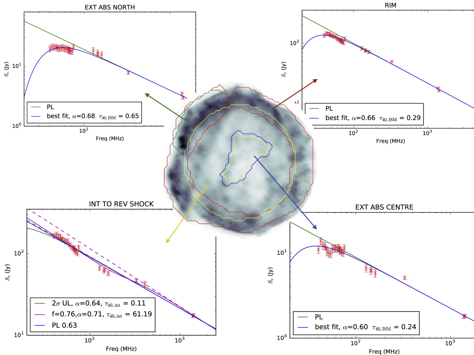
Figure 6. from Low-frequency Radio Absorption in Tycho's Supernova Remnant null 2019 AJ 158 253 doi:10.3847/1538-3881/ab4f80 https://dx.doi.org/10.3847/1538-3881/ab4f80 © 2019. The American Astronomical Society. All rights reserved.
