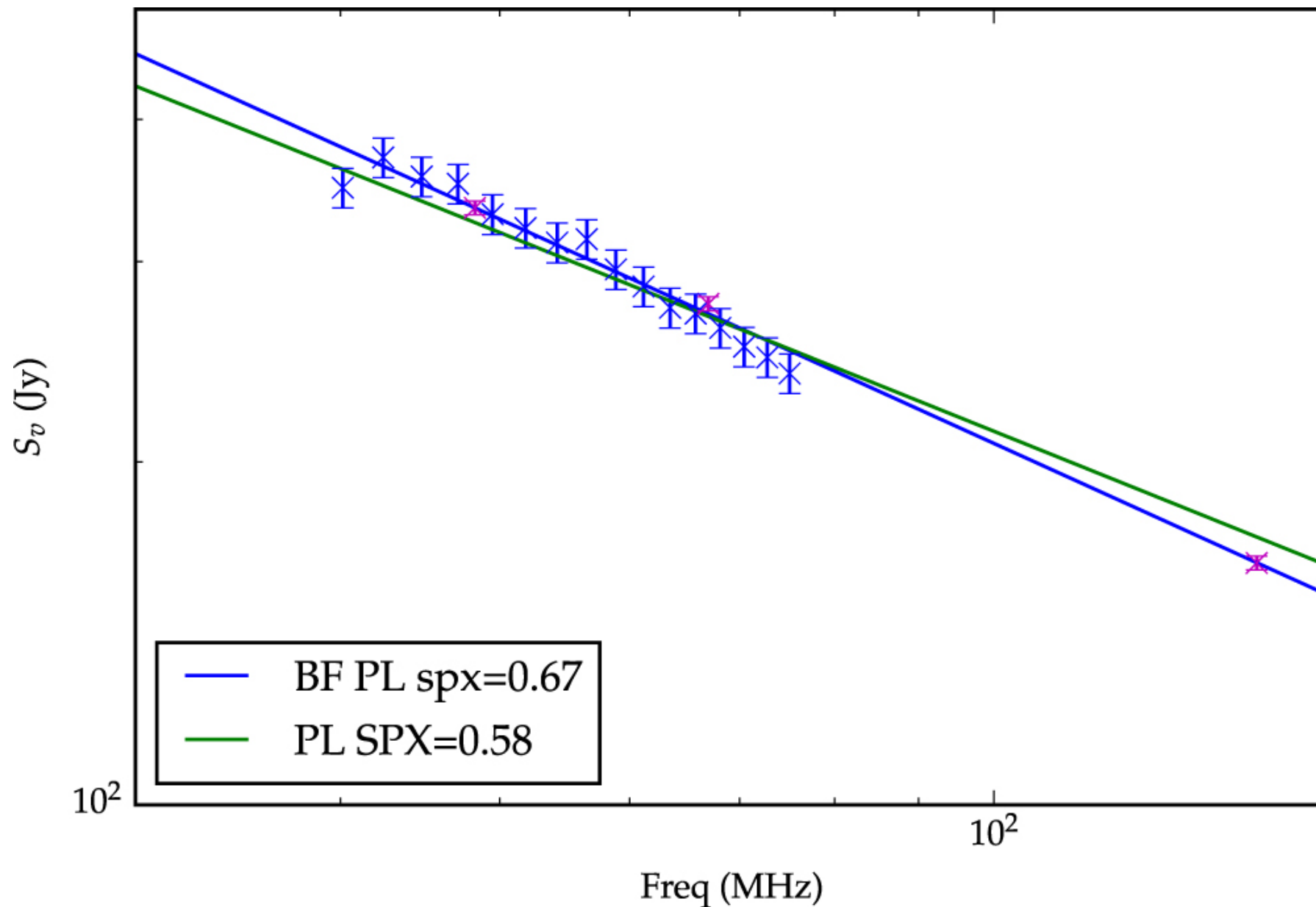
Figure 4. from Low-frequency Radio Absorption in Tycho's Supernova Remnant null 2019 AJ 158 253 doi:10.3847/1538-3881/ab4f80 https://dx.doi.org/10.3847/1538-3881/ab4f80 © 2019. The American Astronomical Society. All rights reserved.
