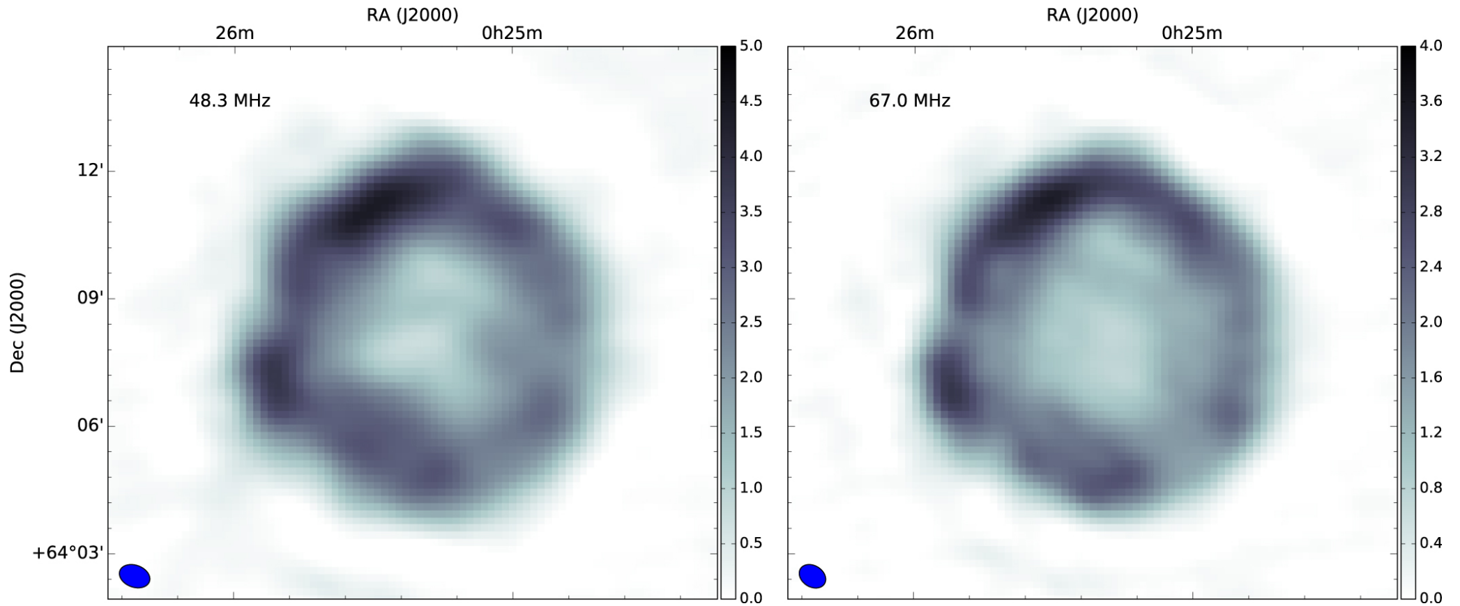
Figure 1. from Low-frequency Radio Absorption in Tycho's Supernova Remnant null 2019 AJ 158 253 doi:10.3847/1538-3881/ab4f80 https://dx.doi.org/10.3847/1538-3881/ab4f80 © 2019. The American Astronomical Society. All rights reserved.
