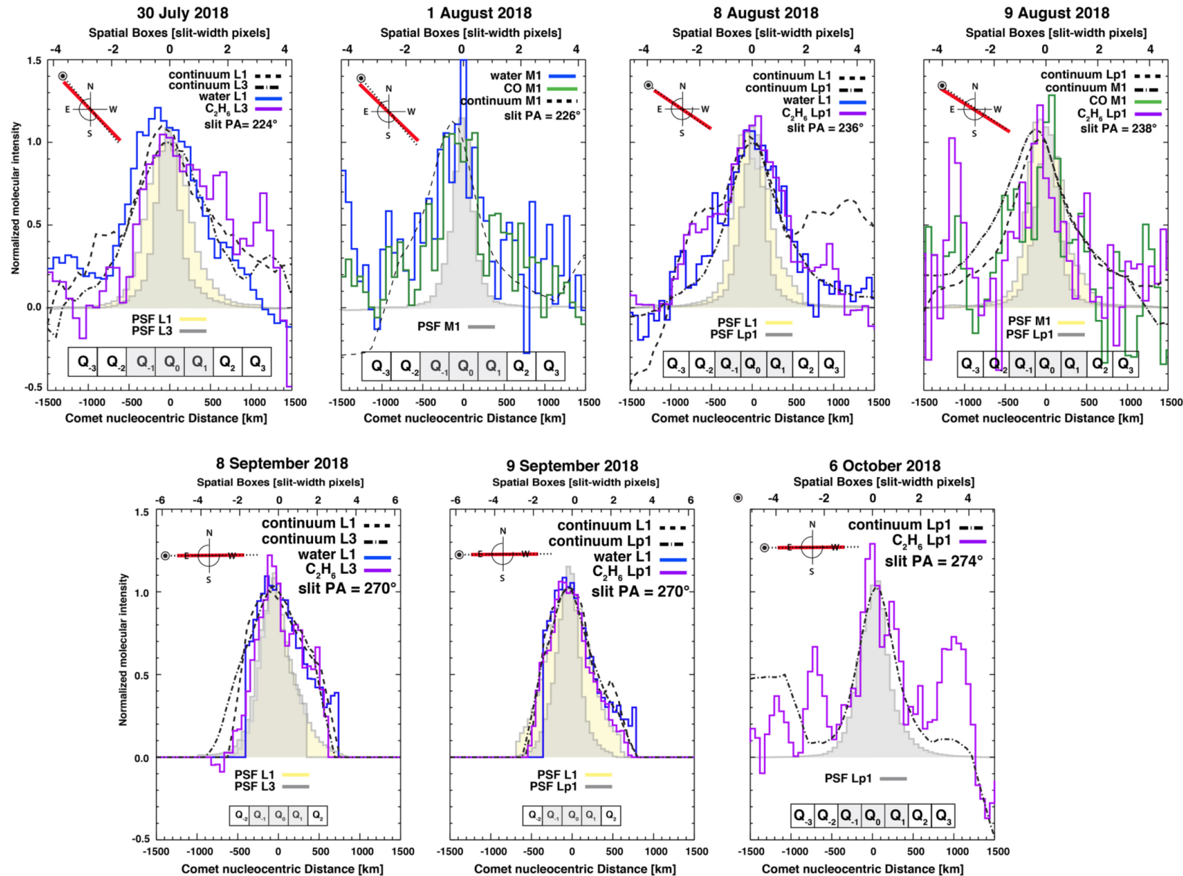
Figure 2. from Quantifying the Evolution of Molecular Production Rates of Comet 21P/Giacobini–Zinner with iSHELL/NASA-IRTF null 2019 AJ 158 254 doi:10.3847/1538-3881/ab4f6e https://dx.doi.org/10.3847/1538-3881/ab4f6e © 2019. The American Astronomical Society. All rights reserved.
