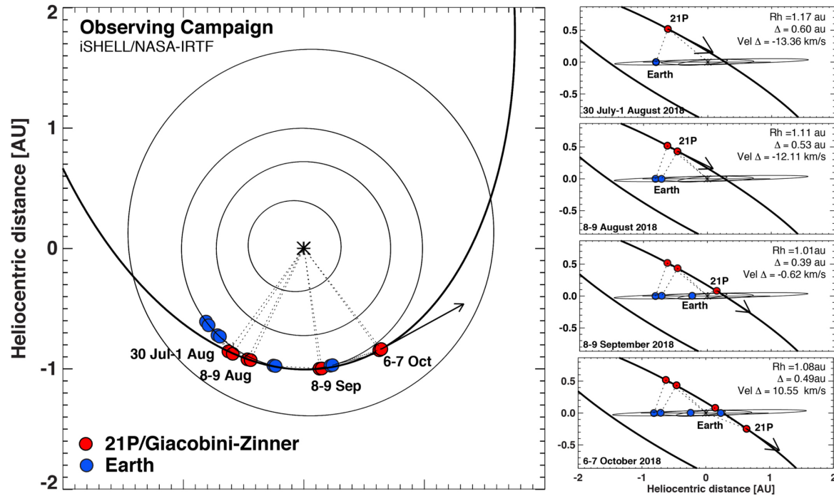
Figure 1. from Quantifying the Evolution of Molecular Production Rates of Comet 21P/Giacobini–Zinner with iSHELL/NASA-IRTF null 2019 AJ 158 254 doi:10.3847/1538-3881/ab4f6e https://dx.doi.org/10.3847/1538-3881/ab4f6e © 2019. The American Astronomical Society. All rights reserved.
