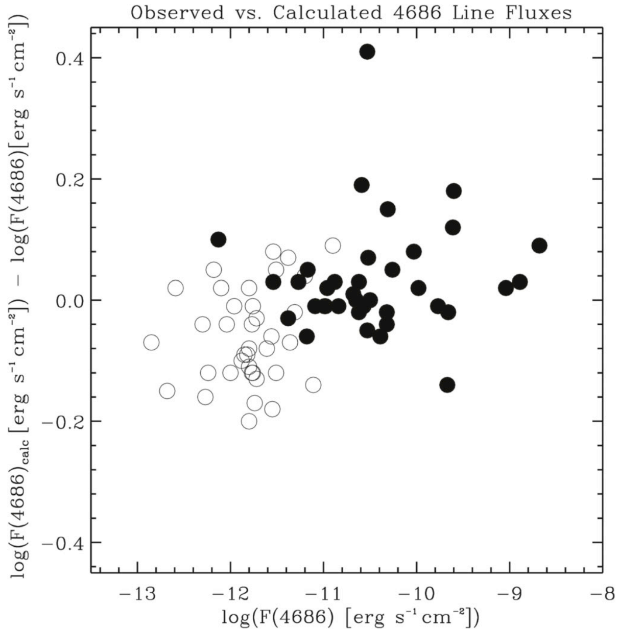
Figure 6. from He II Emission from Wolf-Rayet Stars as a Tool for Measuring Dust Reddening null 2019 AJ 158 192 doi:10.3847/1538-3881/ab44c0 https://dx.doi.org/10.3847/1538-3881/ab44c0 © 2019. The American Astronomical Society. All rights reserved.
