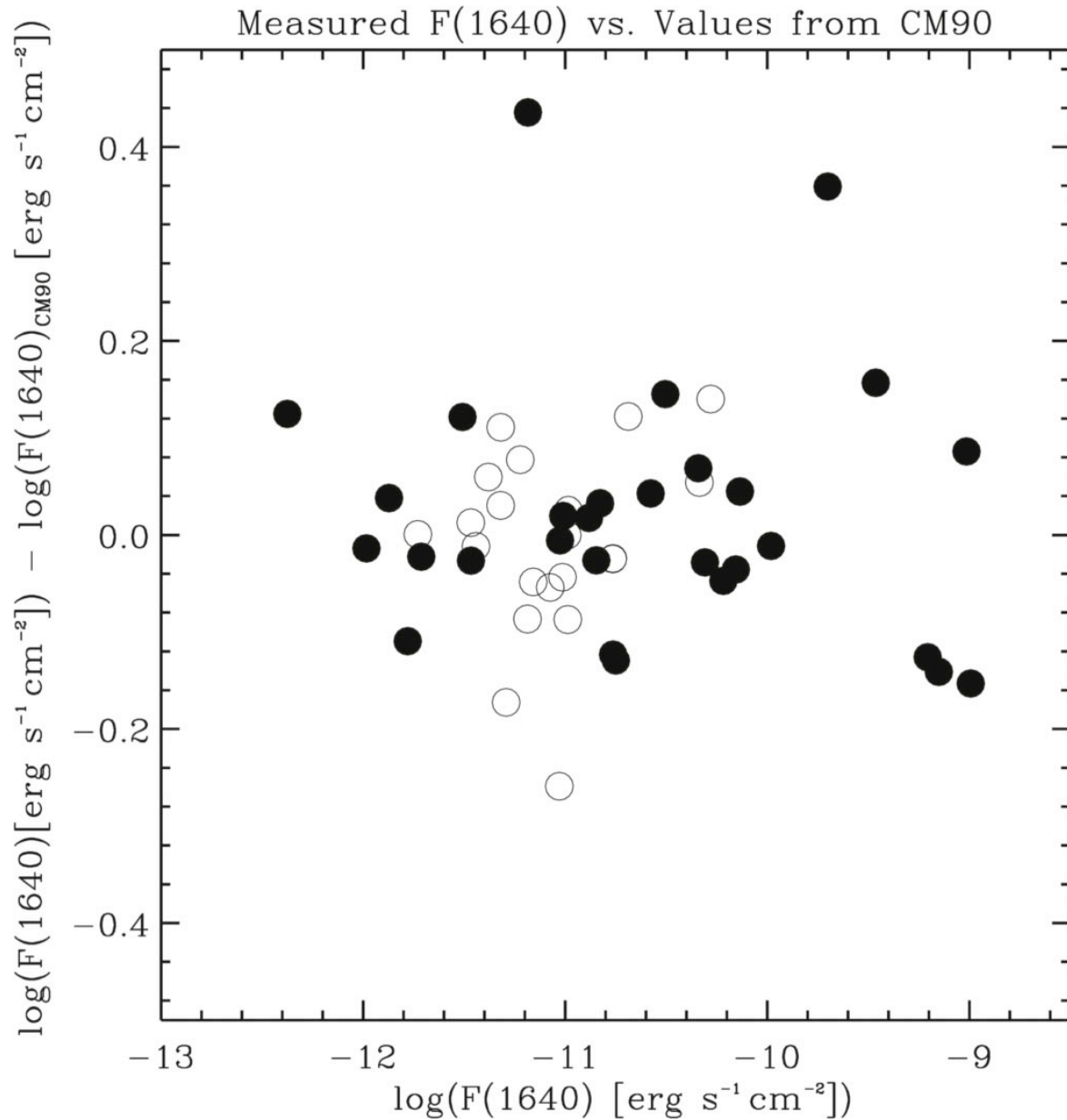
Figure 4. from He II Emission from Wolf-Rayet Stars as a Tool for Measuring Dust Reddening null 2019 AJ 158 192 doi:10.3847/1538-3881/ab44c0 https://dx.doi.org/10.3847/1538-3881/ab44c0 © 2019. The American Astronomical Society. All rights reserved.
