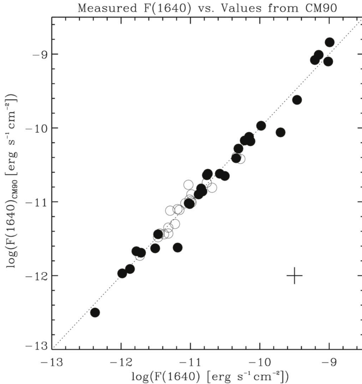
Figure 3. from He II Emission from Wolf-Rayet Stars as a Tool for Measuring Dust Reddening null 2019 AJ 158 192 doi:10.3847/1538-3881/ab44c0 https://dx.doi.org/10.3847/1538-3881/ab44c0 © 2019. The American Astronomical Society. All rights reserved.
