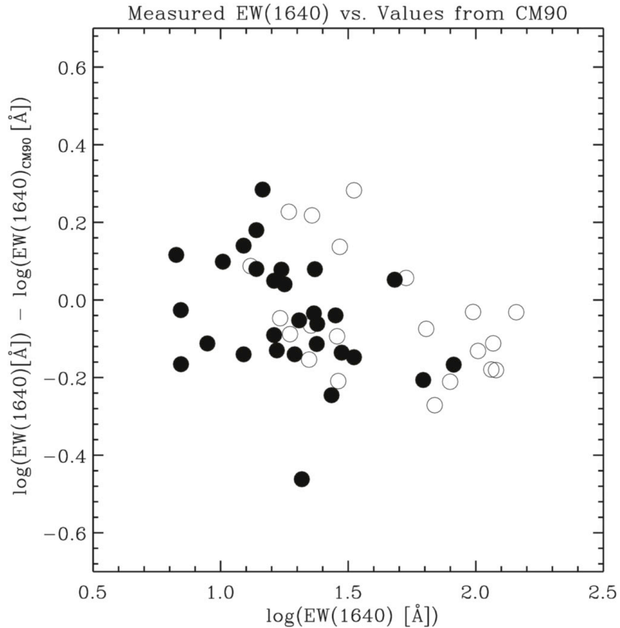
Figure 2. from He II Emission from Wolf–Rayet Stars as a Tool for Measuring Dust Reddening null 2019 AJ 158 192 doi:10.3847/1538-3881/ab44c0 https://dx.doi.org/10.3847/1538-3881/ab44c0 © 2019. The American Astronomical Society. All rights reserved.
