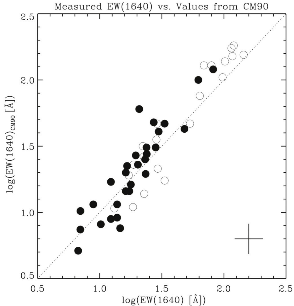
Figure 1. from He II Emission from Wolf-Rayet Stars as a Tool for Measuring Dust Reddening null 2019 AJ 158 192 doi:10.3847/1538-3881/ab44c0 https://dx.doi.org/10.3847/1538-3881/ab44c0 © 2019. The American Astronomical Society. All rights reserved.
