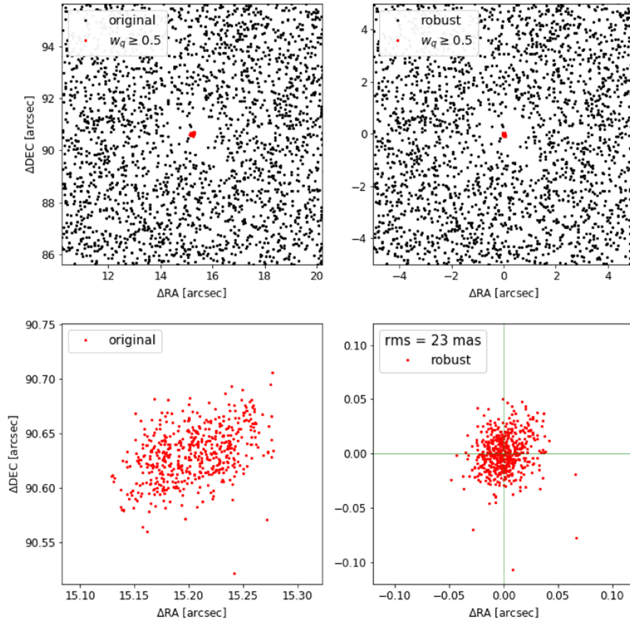
Figure 5. from Robust Registration of Astronomy Catalogs with Applications to the Hubble Space Telescope null 2019 AJ 158 191 doi:10.3847/1538-3881/ab3f38 https://dx.doi.org/10.3847/1538-3881/ab3f38 © 2019. The American Astronomical Society. All rights reserved.
