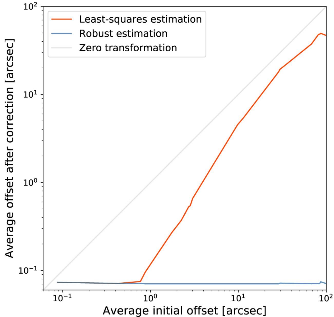
Figure 4. from Robust Registration of Astronomy Catalogs with Applications to the Hubble Space Telescope null 2019 AJ 158 191 doi:10.3847/1538-3881/ab3f38 https://dx.doi.org/10.3847/1538-3881/ab3f38 © 2019. The American Astronomical Society. All rights reserved.
