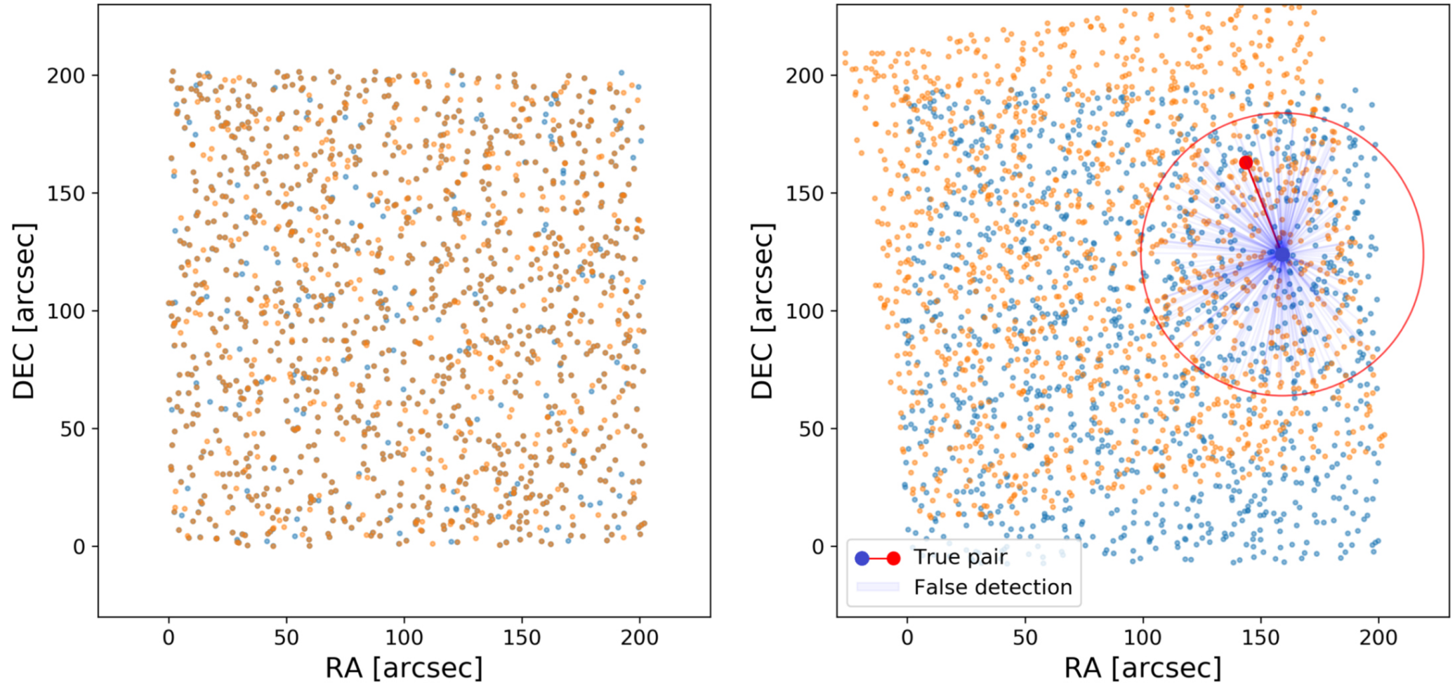
Figure 2. from Robust Registration of Astronomy Catalogs with Applications to the Hubble Space Telescope null 2019 AJ 158 191 doi:10.3847/1538-3881/ab3f38 https://dx.doi.org/10.3847/1538-3881/ab3f38 © 2019. The American Astronomical Society. All rights reserved.
