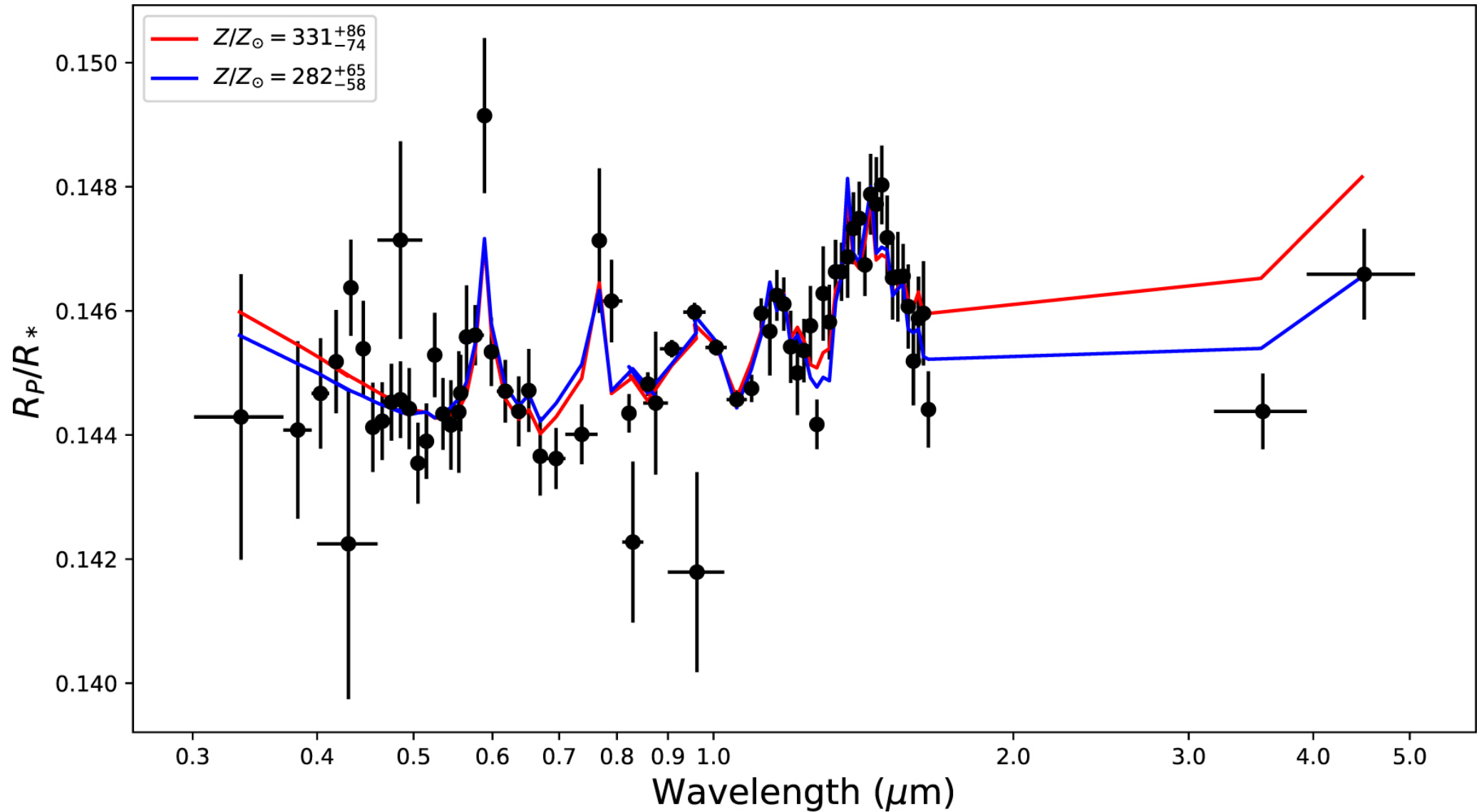
Figure 9. from LRG-BEASTS: Transmission Spectroscopy and Retrieval Analysis of the Highly Inflated Saturn-mass Planet WASP-39b null 2019 AJ 158 144 doi:10.3847/1538-3881/ab397d https://dx.doi.org/10.3847/1538-3881/ab397d © 2019. The American Astronomical Society. All rights reserved.
