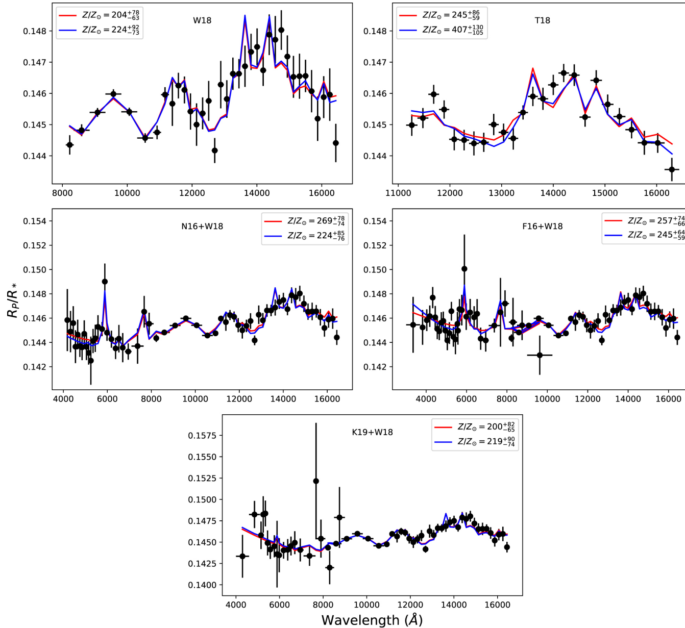
Figure 8. from LRG-BEASTS: Transmission Spectroscopy and Retrieval Analysis of the Highly Inflated Saturn-mass Planet WASP-39b null 2019 AJ 158 144 doi:10.3847/1538-3881/ab397d https://dx.doi.org/10.3847/1538-3881/ab397d © 2019. The American Astronomical Society. All rights reserved.
