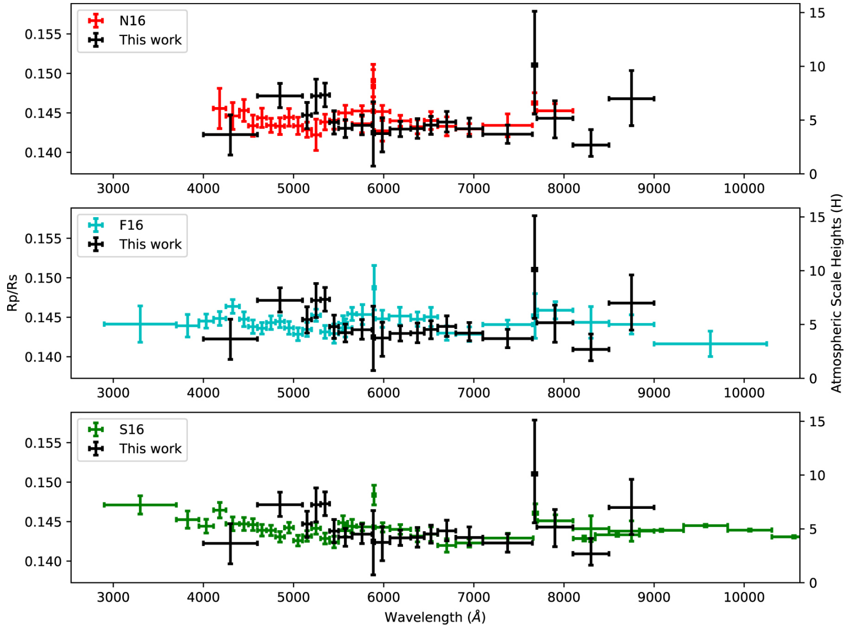
Figure 7. from LRG-BEASTS: Transmission Spectroscopy and Retrieval Analysis of the Highly Inflated Saturn-mass Planet WASP-39b null 2019 AJ 158 144 doi:10.3847/1538-3881/ab397d https://dx.doi.org/10.3847/1538-3881/ab397d © 2019. The American Astronomical Society. All rights reserved.
