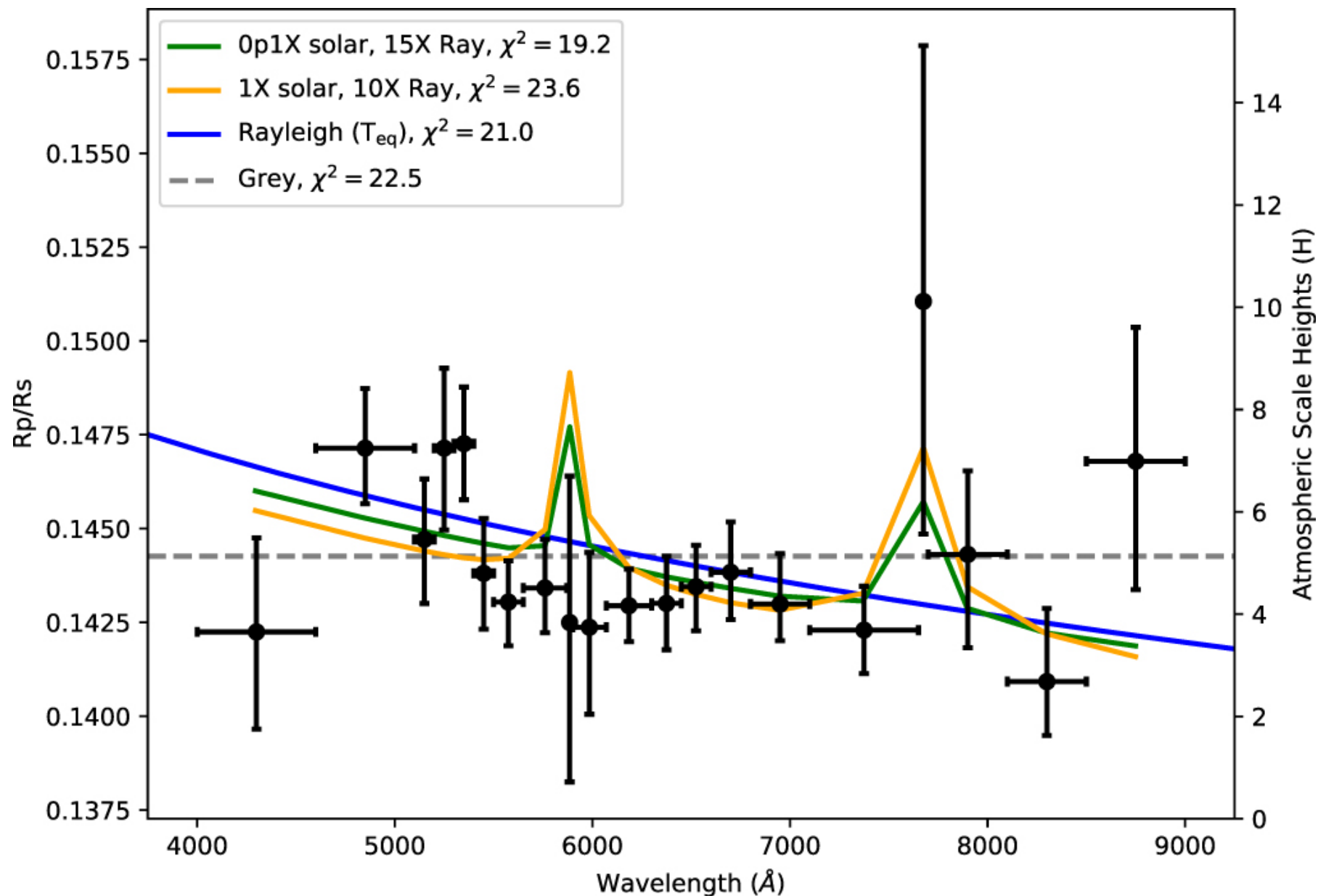
Figure 6. from LRG-BEASTS: Transmission Spectroscopy and Retrieval Analysis of the Highly Inflated Saturn-mass Planet WASP-39b null 2019 AJ 158 144 doi:10.3847/1538-3881/ab397d https://dx.doi.org/10.3847/1538-3881/ab397d © 2019. The American Astronomical Society. All rights reserved.
