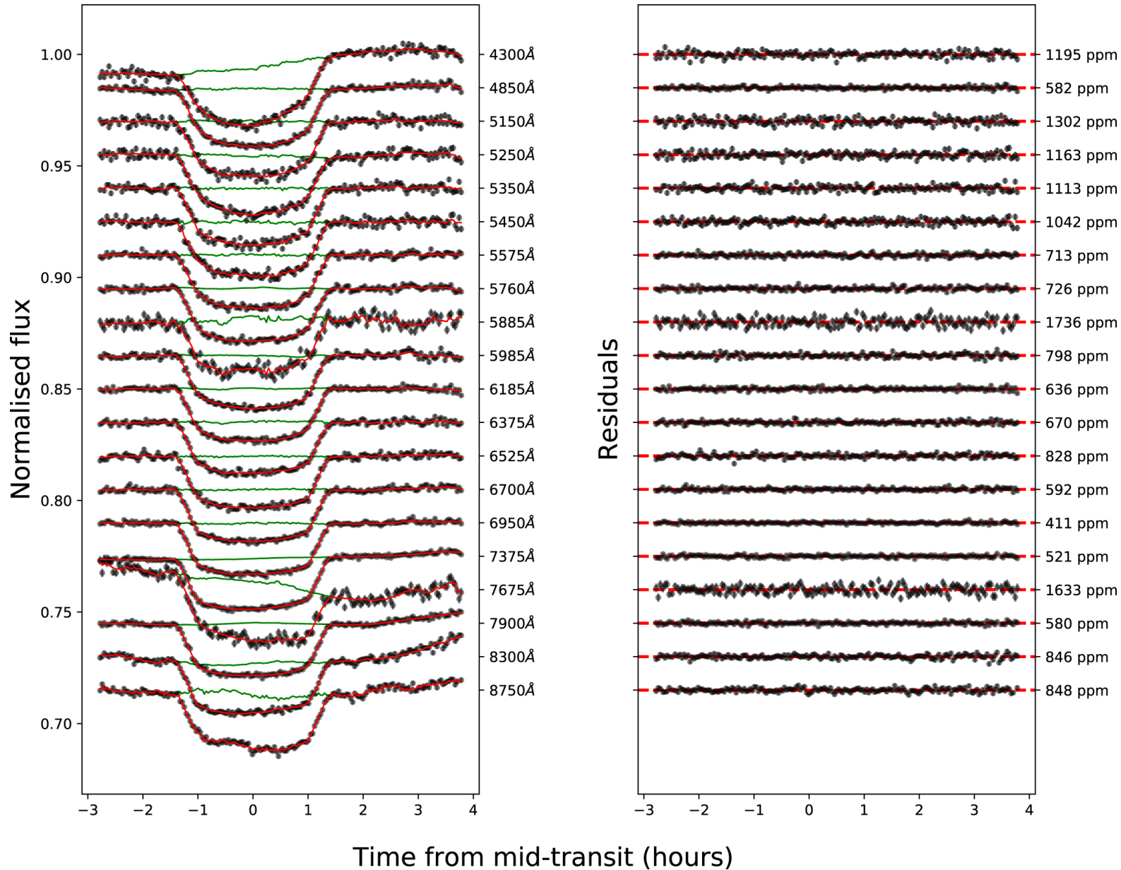
Figure 5. from LRG-BEASTS: Transmission Spectroscopy and Retrieval Analysis of the Highly Inflated Saturn-mass Planet WASP-39b null 2019 AJ 158 144 doi:10.3847/1538-3881/ab397d https://dx.doi.org/10.3847/1538-3881/ab397d © 2019. The American Astronomical Society. All rights reserved.
