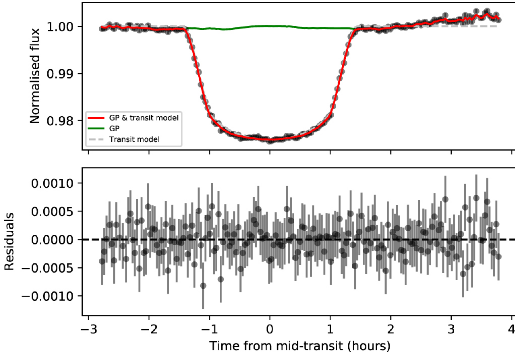
Figure 4. from LRG-BEASTS: Transmission Spectroscopy and Retrieval Analysis of the Highly Inflated Saturn-mass Planet WASP-39b null 2019 AJ 158 144 doi:10.3847/1538-3881/ab397d https://dx.doi.org/10.3847/1538-3881/ab397d © 2019. The American Astronomical Society. All rights reserved.
