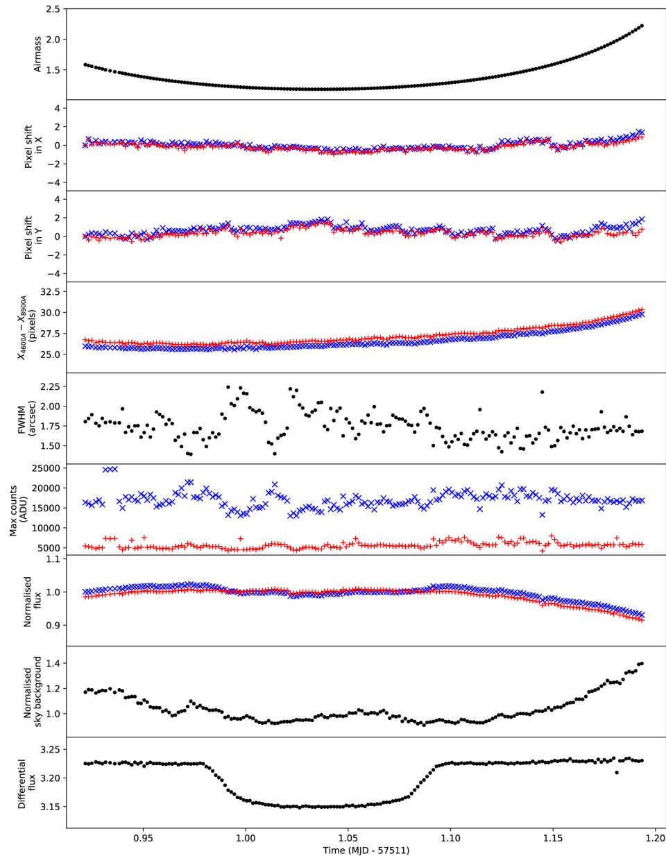
Figure 2. from LRG-BEASTS: Transmission Spectroscopy and Retrieval Analysis of the Highly Inflated Saturn-mass Planet WASP-39b null 2019 AJ 158 144 doi:10.3847/1538-3881/ab397d https://dx.doi.org/10.3847/1538-3881/ab397d © 2019. The American Astronomical Society. All rights reserved.
