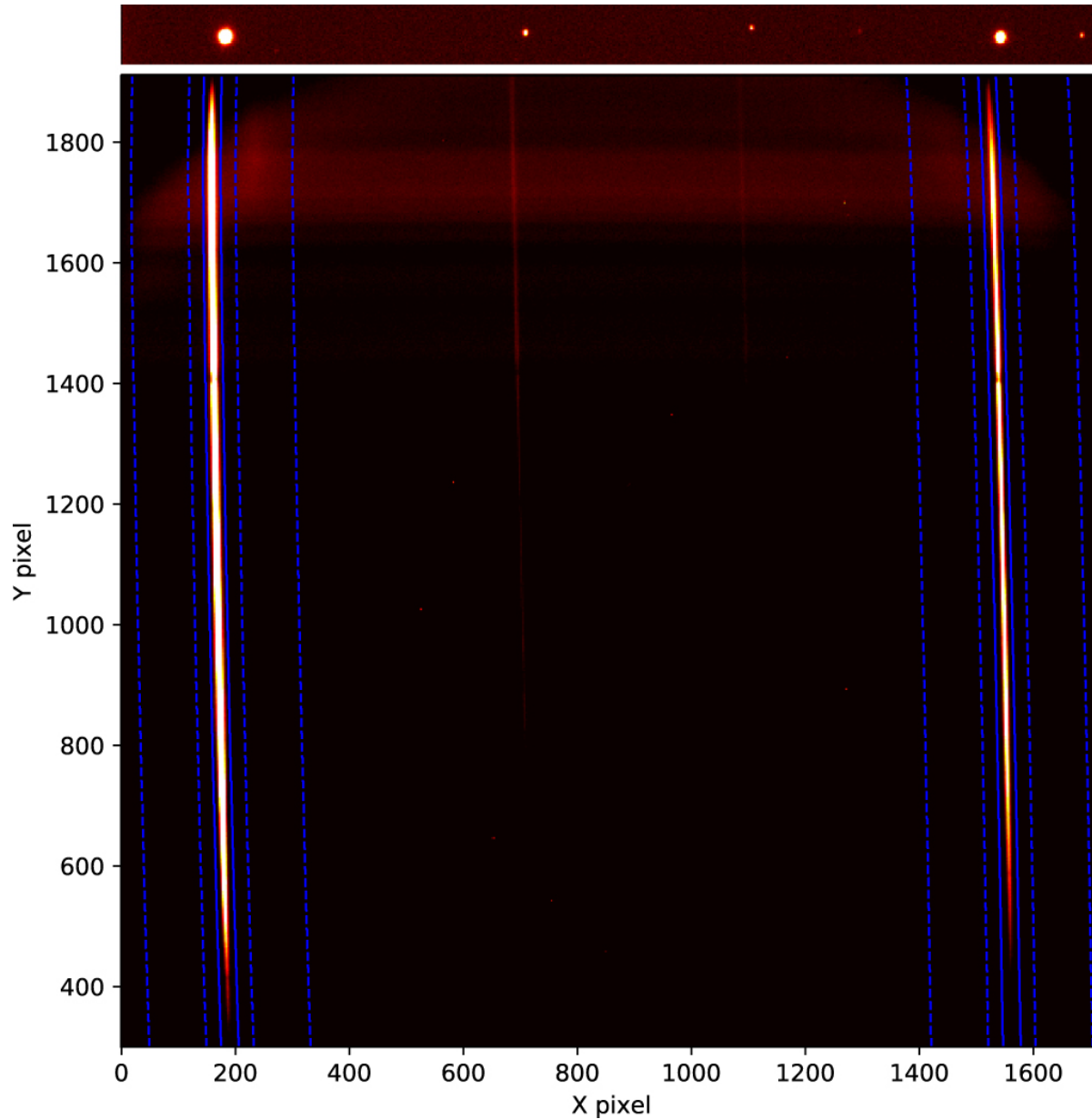
Figure 1. from LRG-BEASTS: Transmission Spectroscopy and Retrieval Analysis of the Highly Inflated Saturn-mass Planet WASP-39b null 2019 AJ 158 144 doi:10.3847/1538-3881/ab397d https://dx.doi.org/10.3847/1538-3881/ab397d © 2019. The American Astronomical Society. All rights reserved.
