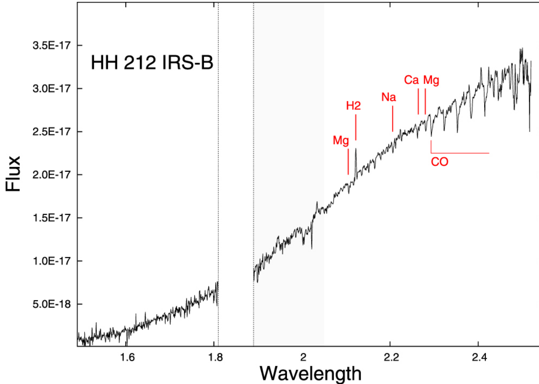
Figure 8. from The Giant Herbig–Haro Flow HH 212 and Associated Star Formation null 2019 AJ 158 107 doi:10.3847/1538-3881/ab2d25 https://dx.doi.org/10.3847/1538-3881/ab2d25 © 2019. The American Astronomical Society. All rights reserved.
