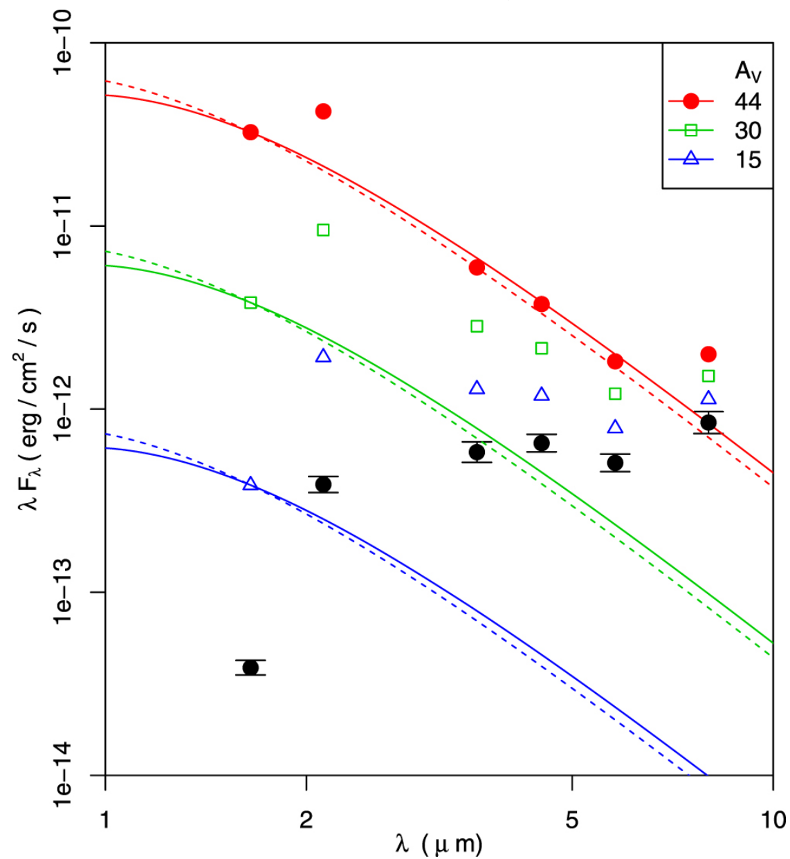
Figure 7. from The Giant Herbig–Haro Flow HH 212 and Associated Star Formation null 2019 AJ 158 107 doi:10.3847/1538-3881/ab2d25 https://dx.doi.org/10.3847/1538-3881/ab2d25 © 2019. The American Astronomical Society. All rights reserved.
