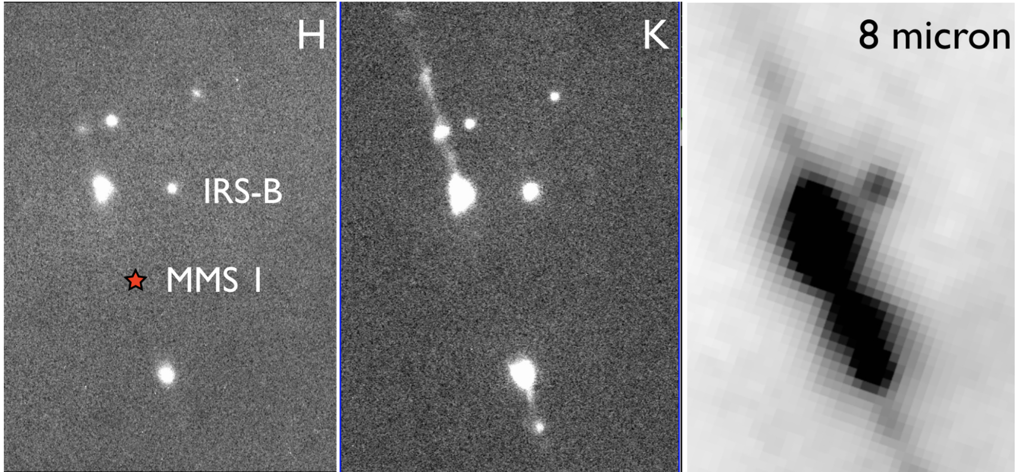
Figure 6. from The Giant Herbig–Haro Flow HH 212 and Associated Star Formation null 2019 AJ 158 107 doi:10.3847/1538-3881/ab2d25 https://dx.doi.org/10.3847/1538-3881/ab2d25 © 2019. The American Astronomical Society. All rights reserved.
