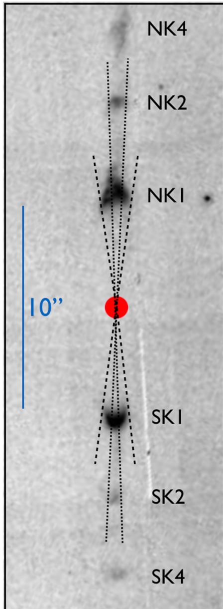
Figure 5. from The Giant Herbig–Haro Flow HH 212 and Associated Star Formation null 2019 AJ 158 107 doi:10.3847/1538-3881/ab2d25 http://dx.doi.org/10.3847/1538-3881/ab2d25 © 2019. The American Astronomical Society. All rights reserved.
