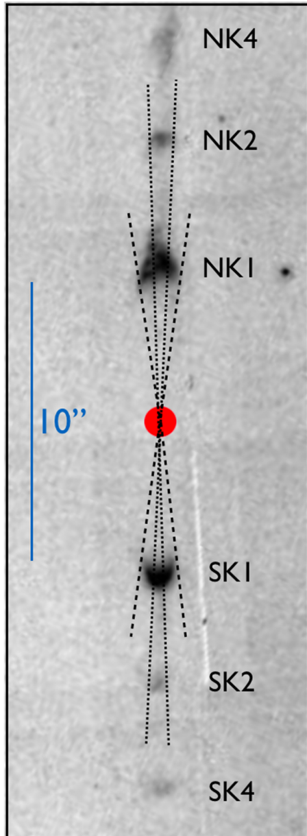
Figure 5. from The Giant Herbig–Haro Flow HH 212 and Associated Star Formation null 2019 AJ 158 107 doi:10.3847/1538-3881/ab2d25 https://dx.doi.org/10.3847/1538-3881/ab2d25 © 2019. The American Astronomical Society. All rights reserved.
