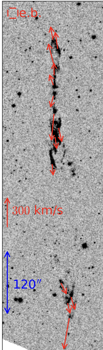
Figure 4. from The Giant Herbig–Haro Flow HH 212 and Associated Star Formation null 2019 AJ 158 107 doi:10.3847/1538-3881/ab2d25 http://dx.doi.org/10.3847/1538-3881/ab2d25 © 2019. The American Astronomical Society. All rights reserved.
