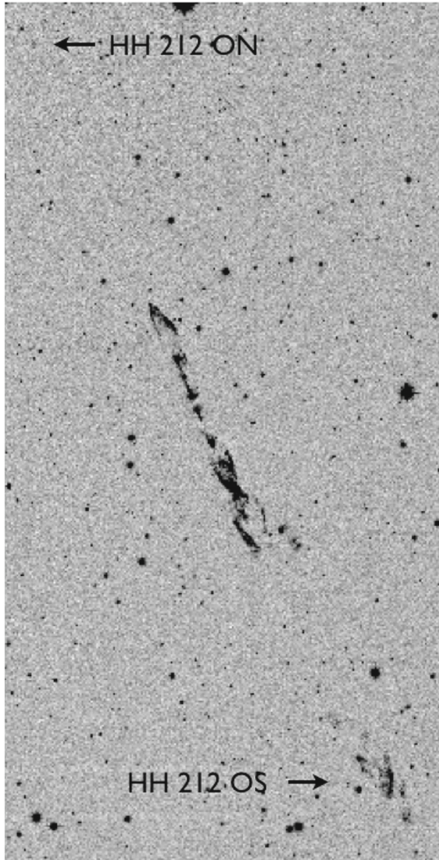
Figure 1. from The Giant Herbig–Haro Flow HH 212 and Associated Star Formation null 2019 AJ 158 107 doi:10.3847/1538-3881/ab2d25 https://dx.doi.org/10.3847/1538-3881/ab2d25 © 2019. The American Astronomical Society. All rights reserved.
