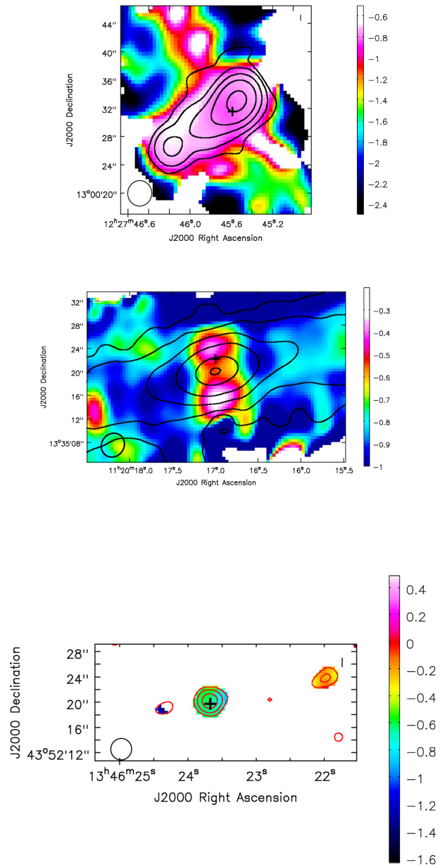
Figure 4. from CHANG-ES. XX. High-resolution Radio Continuum Images of Edge-on Galaxies and Their AGNs: Data Release 3 null 2019 AJ 158 21 doi:10.3847/1538-3881/ab25f6 http://dx.doi.org/10.3847/1538-3881/ab25f6 © 2019. The American Astronomical Society. All rights reserved.
