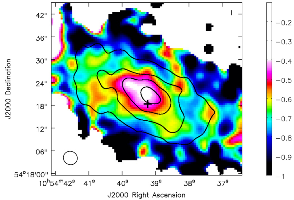
Figure 3. from CHANG-ES. XX. High-resolution Radio Continuum Images of Edge-on Galaxies and Their AGNs: Data Release 3 null 2019 AJ 158 21 doi:10.3847/1538-3881/ab25f6 https://dx.doi.org/10.3847/1538-3881/ab25f6 © 2019. The American Astronomical Society. All rights reserved.
