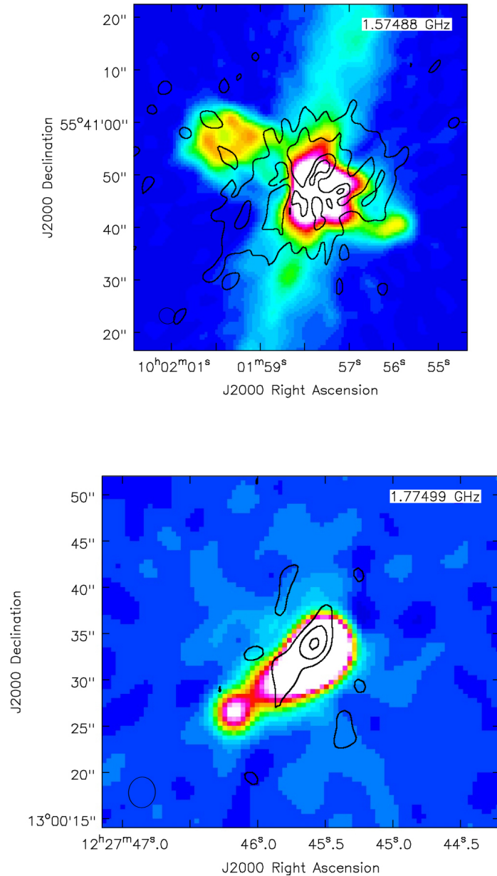
Figure 2. from CHANG-ES. XX. High-resolution Radio Continuum Images of Edge-on Galaxies and Their AGNs: Data Release 3 null 2019 AJ 158 21 doi:10.3847/1538-3881/ab25f6 https://dx.doi.org/10.3847/1538-3881/ab25f6 © 2019. The American Astronomical Society. All rights reserved.
