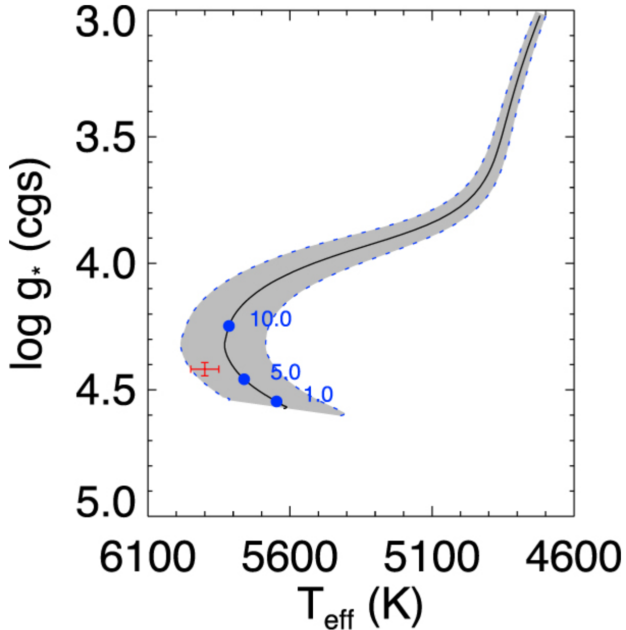
Figure 8. from KELT-23Ab: A Hot Jupiter Transiting a Near-solar Twin Close to the TESS and JWST Continuous Viewing Zones null 2019 AJ 158 78 doi:10.3847/1538-3881/ab24c7 https://dx.doi.org/10.3847/1538-3881/ab24c7 © 2019. The American Astronomical Society. All rights reserved.
