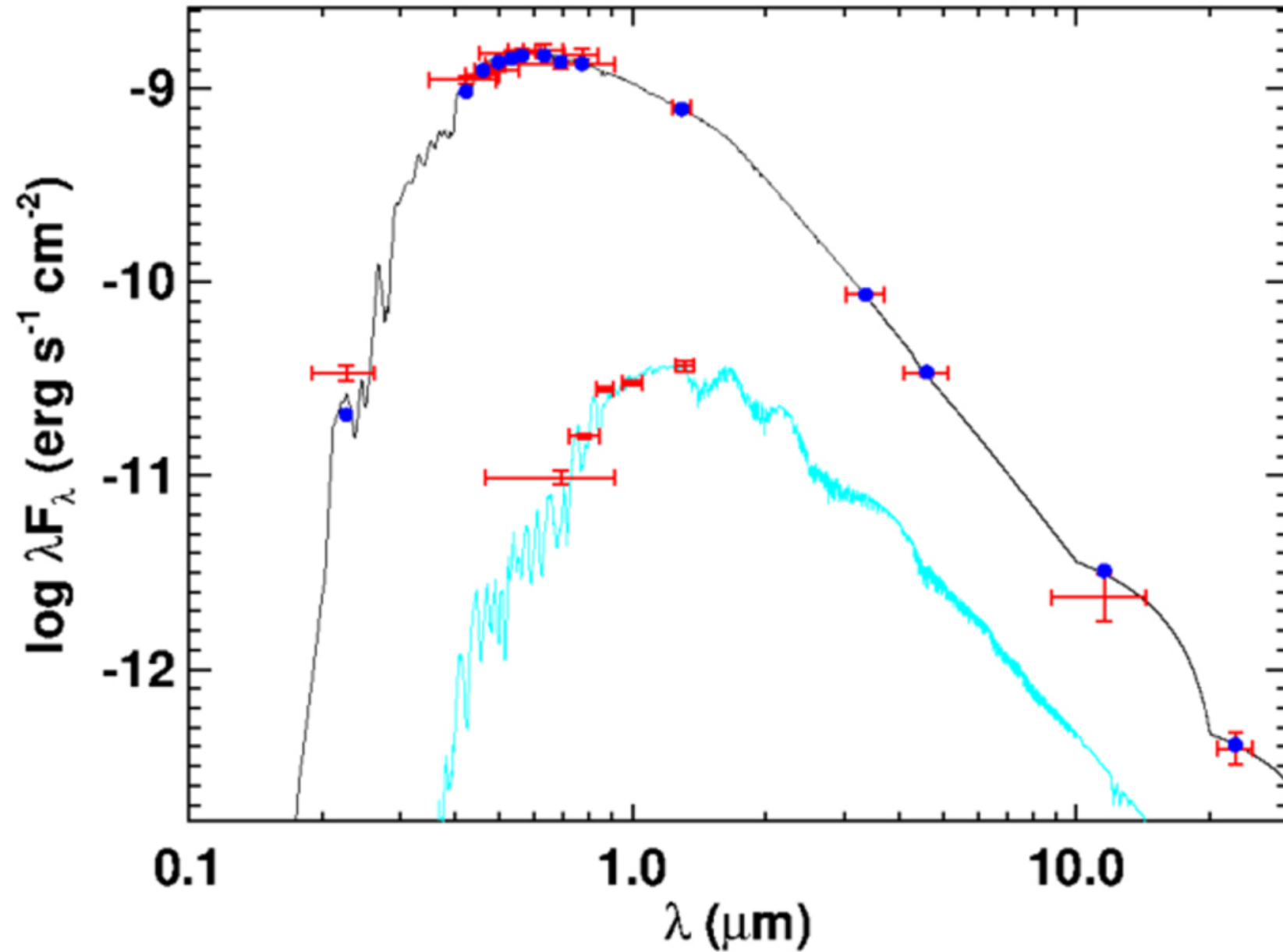
Figure 7. from KELT-23Ab: A Hot Jupiter Transiting a Near-solar Twin Close to the TESS and JWST Continuous Viewing Zones null 2019 AJ 158 78 doi:10.3847/1538-3881/ab24c7 https://dx.doi.org/10.3847/1538-3881/ab24c7 © 2019. The American Astronomical Society. All rights reserved.
