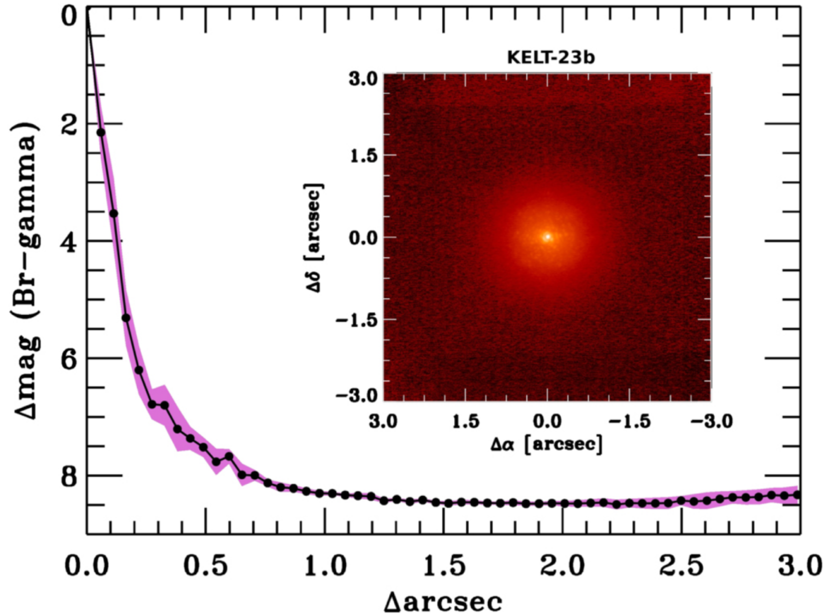
Figure 6. from KELT-23Ab: A Hot Jupiter Transiting a Near-solar Twin Close to the TESS and JWST Continuous Viewing Zones null 2019 AJ 158 78 doi:10.3847/1538-3881/ab24c7 https://dx.doi.org/10.3847/1538-3881/ab24c7 © 2019. The American Astronomical Society. All rights reserved.
