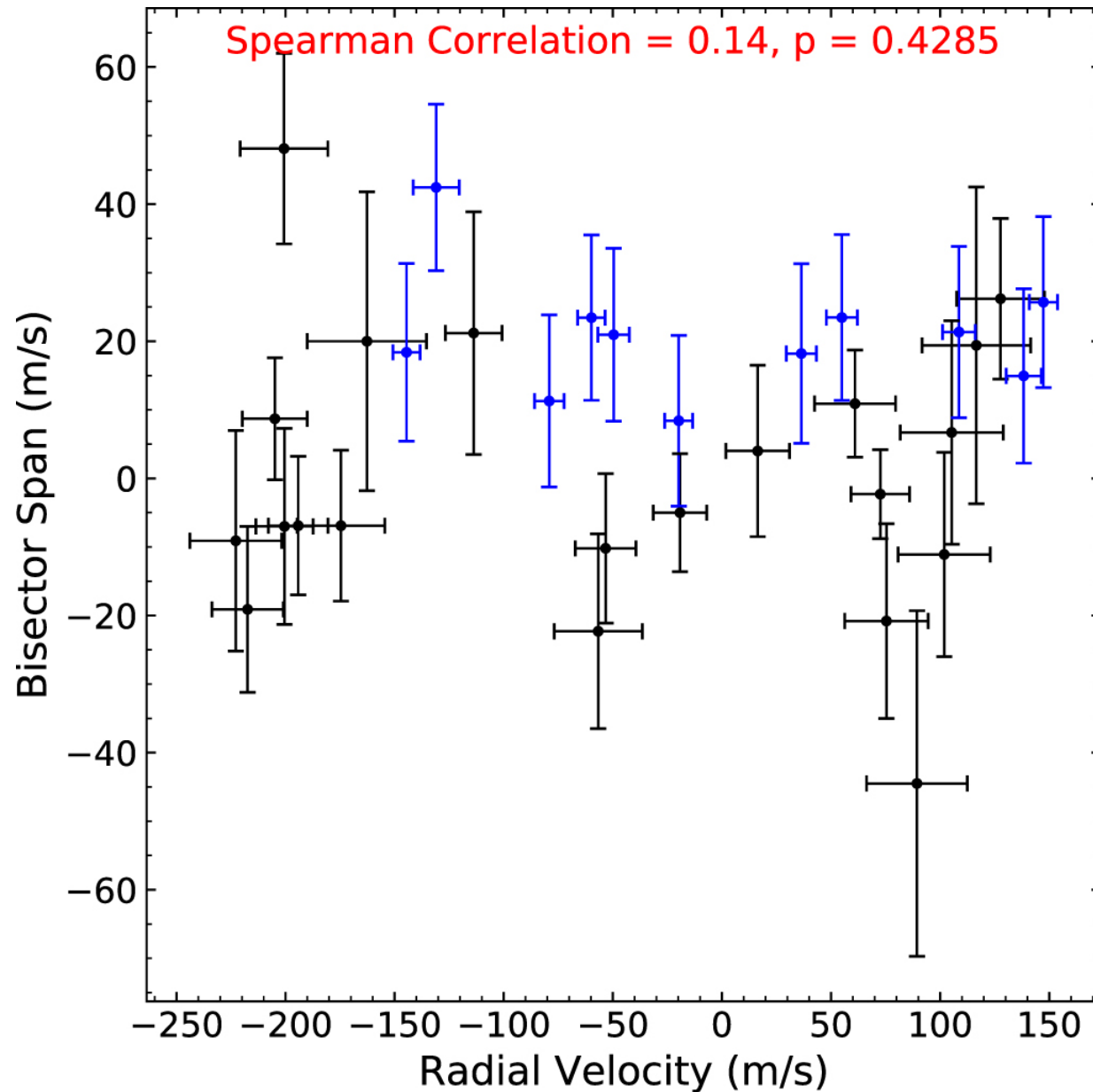
Figure 4. from KELT-23Ab: A Hot Jupiter Transiting a Near-solar Twin Close to the TESS and JWST Continuous Viewing Zones null 2019 AJ 158 78 doi:10.3847/1538-3881/ab24c7 https://dx.doi.org/10.3847/1538-3881/ab24c7 © 2019. The American Astronomical Society. All rights reserved.
