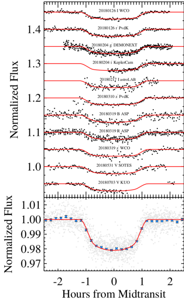
Figure 2. from KELT-23Ab: A Hot Jupiter Transiting a Near-solar Twin Close to the TESS and JWST Continuous Viewing Zones null 2019 AJ 158 78 doi:10.3847/1538-3881/ab24c7 https://dx.doi.org/10.3847/1538-3881/ab24c7 © 2019. The American Astronomical Society. All rights reserved.
