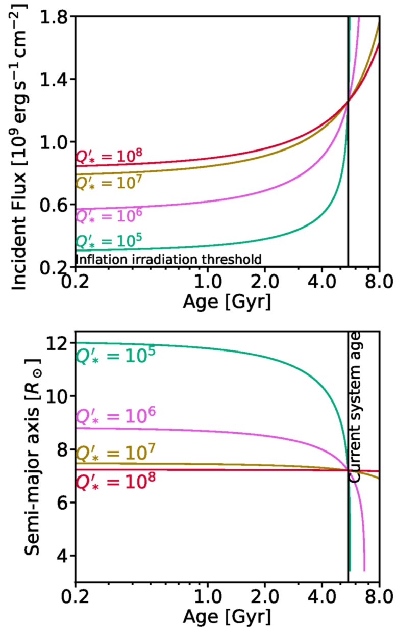
Figure 10. from KELT-23Ab: A Hot Jupiter Transiting a Near-solar Twin Close to the TESS and JWST Continuous Viewing Zones null 2019 AJ 158 78 doi:10.3847/1538-3881/ab24c7 https://dx.doi.org/10.3847/1538-3881/ab24c7 © 2019. The American Astronomical Society. All rights reserved.
