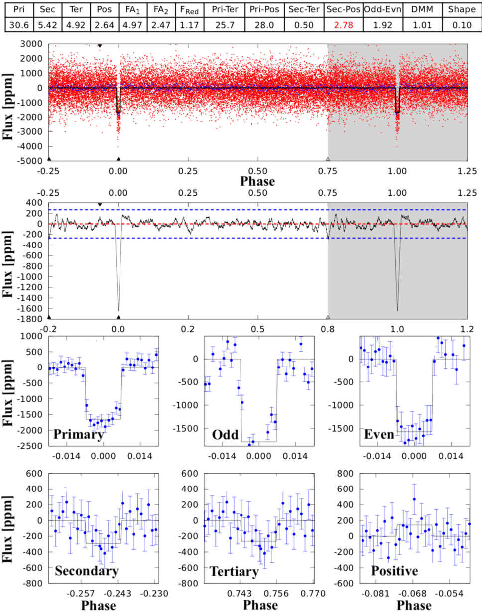
Figure 6. from The L 98-59 System: Three Transiting, Terrestrial-size Planets Orbiting a Nearby M Dwarf null 2019 AJ 158 32 doi:10.3847/1538-3881/ab2459 https://dx.doi.org/10.3847/1538-3881/ab2459 © 2019. The American Astronomical Society. All rights reserved.
