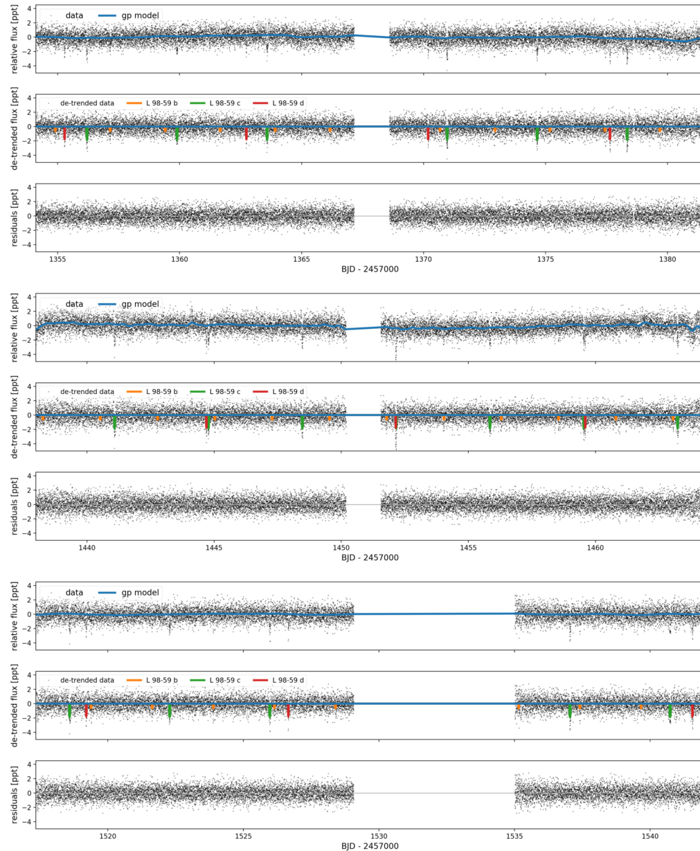
Figure 4. from The L 98-59 System: Three Transiting, Terrestrial-size Planets Orbiting a Nearby M Dwarf null 2019 AJ 158 32 doi:10.3847/1538-3881/ab2459 https://dx.doi.org/10.3847/1538-3881/ab2459 © 2019. The American Astronomical Society. All rights reserved.
