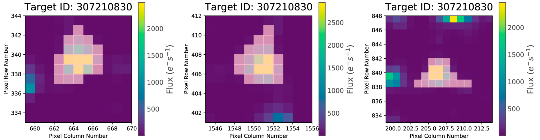
Figure 3. from The L 98-59 System: Three Transiting, Terrestrial-size Planets Orbiting a Nearby M Dwarf null 2019 AJ 158 32 doi:10.3847/1538-3881/ab2459 https://dx.doi.org/10.3847/1538-3881/ab2459 © 2019. The American Astronomical Society. All rights reserved.
