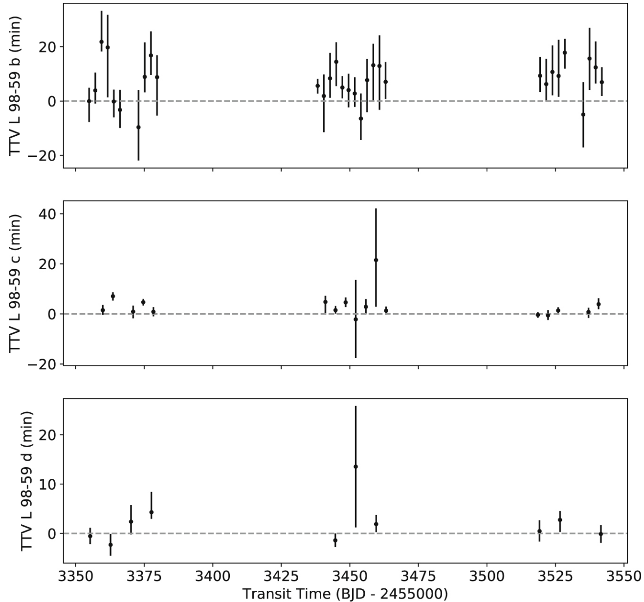
Figure 22. from The L 98-59 System: Three Transiting, Terrestrial-size Planets Orbiting a Nearby M Dwarf null 2019 AJ 158 32 doi:10.3847/1538-3881/ab2459 https://dx.doi.org/10.3847/1538-3881/ab2459 © 2019. The American Astronomical Society. All rights reserved.
